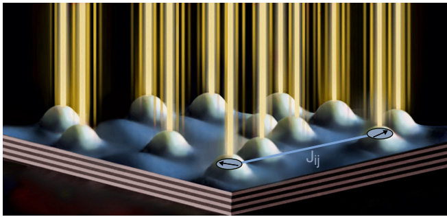
FIG. 2: A general scheme for a gain-dissipative simulator. The condensates are pumped in a two-dimensional lattice with interaction strengths J_{ij} between the adjacent vertices. The final phase configuration minimizes the XY or Ising Hamiltonians depending on a particular physical system.
